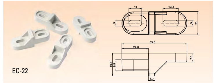
Plastic Wall Mounting Lugs
