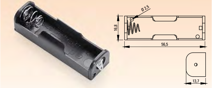
BH-311-1D
