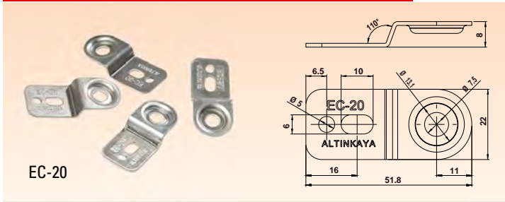
Aluminium Wall Mounting Lugs
