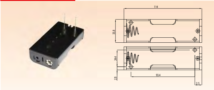
BH-321-1P24
